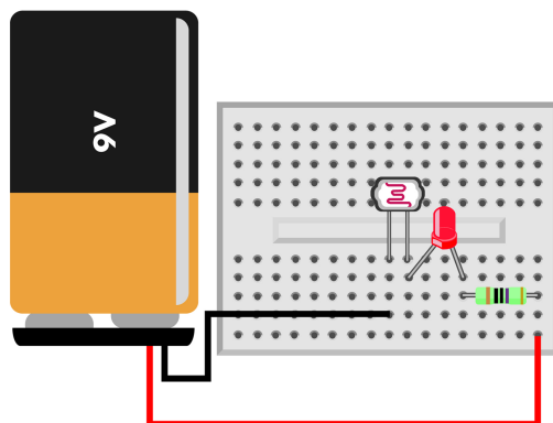
Figure 2-8. LED/LDR circuit
