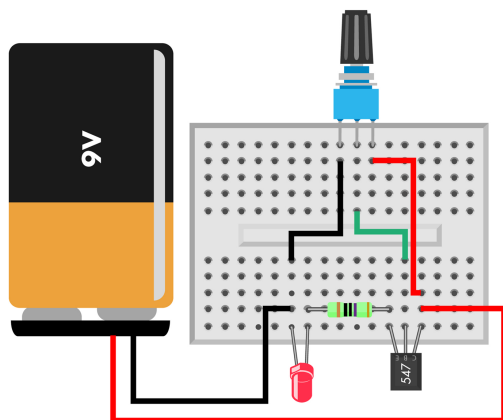
Figure 2-13. Fading an LED with an NPN transistor
