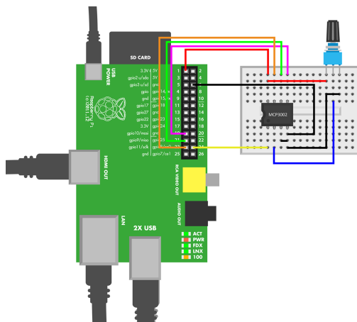
Figure 4-6. Potentiometer connected to Raspberry Pi
